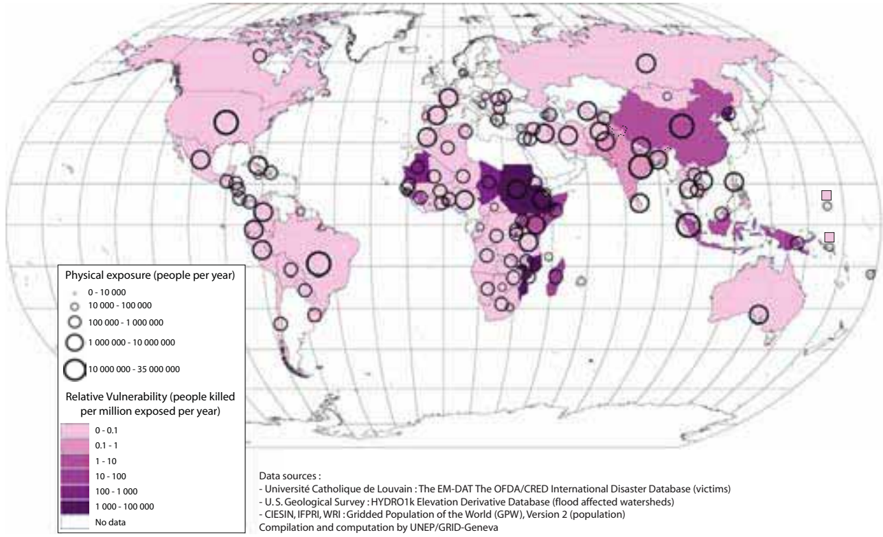
Map 10.2: Physical exposure and relative vulnerability to droughts, 1980-2000
