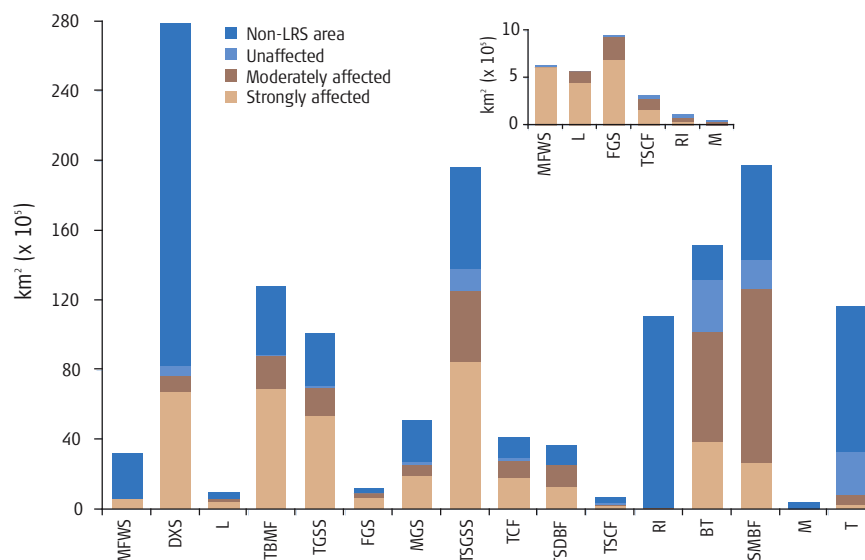
Figure 5.4: Fragmentation and flow regulation by biome type
